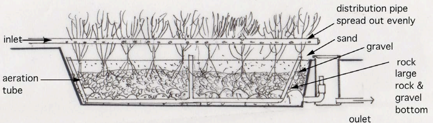
VERTICAL REED BED
